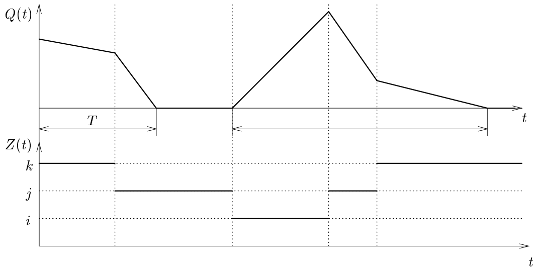
Figure 1: Busy periods of a stochastic fluid model
