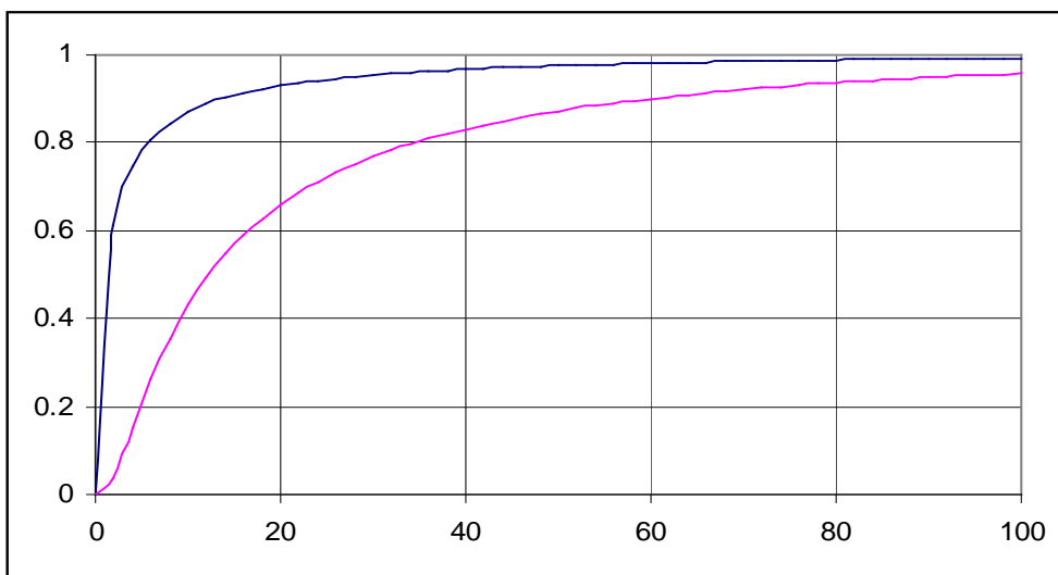
Figure 5: Distribution of the busy period with different initial states
