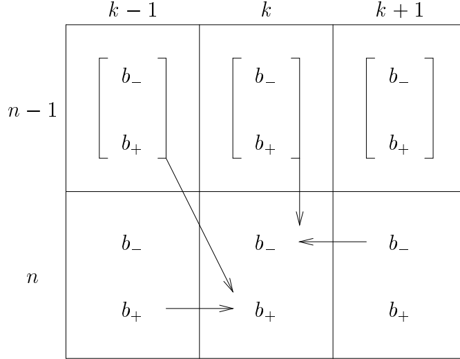
Figure 3: Computation of the b_i(n, k)
