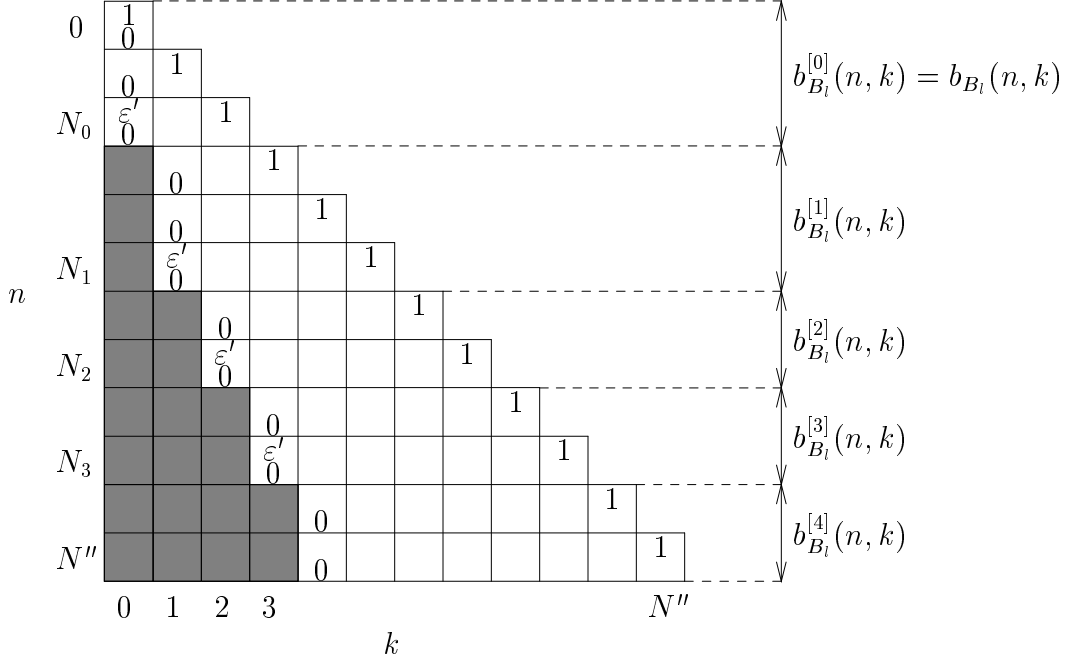
Figure 4: In gray, the cells (n, k) that are not computed
