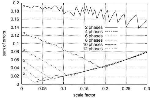
Fig. 22. \epsilon_{SUM} for distribution U2 with 1-phase appr. for exponential durations
