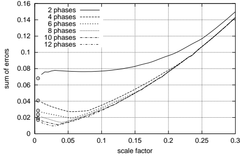
Fig. 20. \epsilon_{SUM} for distribution U1 with 1-phase appr. for exponential durations
