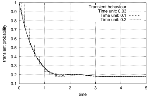
Fig. 26. Approximating transient probabilities
